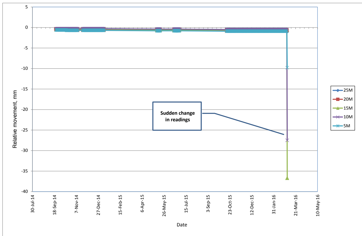
Fig. 18. MPBX data showing abrupt change before the collapse
