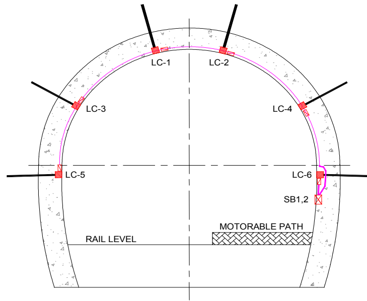
INSTRUMENTATION MONITORING CROSS SECTION (ONE SECTION AT EVERY ALTERNATE 500 m INTERVAL)
